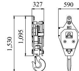
32 t Hook Weight: 500 kg
