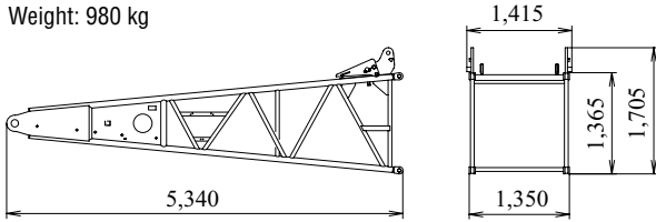
3.0 m Boom Insert Weight: 255 kg
